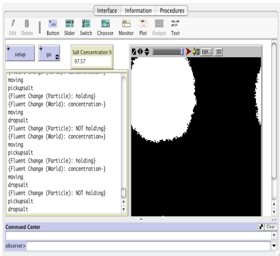
Figure 4: Emergence of single “clump”
